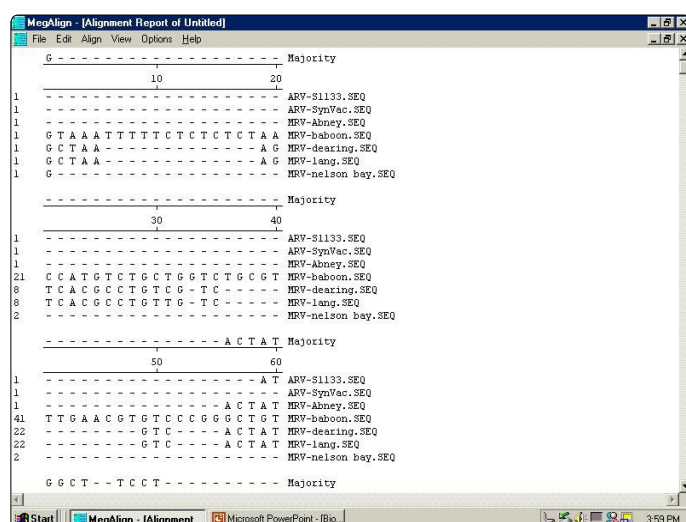
Figure 5. Multiple Alignment of ARV \sigma C with MRV \sigma Sequences
