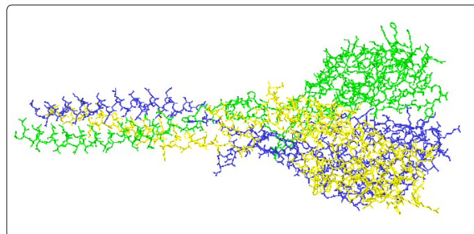
Figure 7. The predicted 3D-structure of the sigma C trimer: Each color chain is a sigmaC monomer. Structure is predicted for the regions from 122 to 316. There is long helix from 124 to 153, which forms the stem region. A loop (154-164) and two anti-parallel beta-sheets regions (165-176, 179-193) for the neck region. The mushroom like head is form by residues 196 to 316. The model is built by homology modeling method using the template of the avian reovirus sigma C 117-326, (PDB 2VRS)
