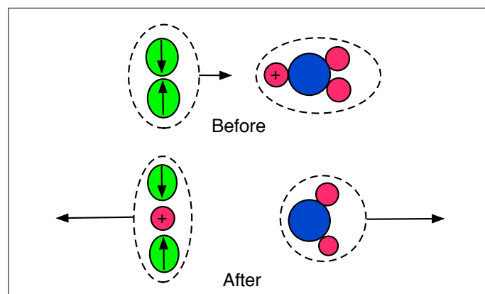
Figure 4. The tresino -formation collision of a Cooper pair and a hydronium ( \text{H}_3\text{O}^+ ) ion.
