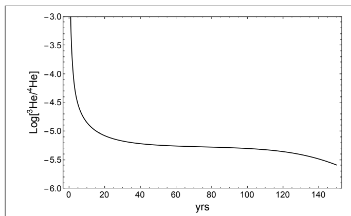
Figure 2. The ratio of ^3\text{He} and ^4\text{He} as a function of time from the numerical integration of the reaction rate equations.
