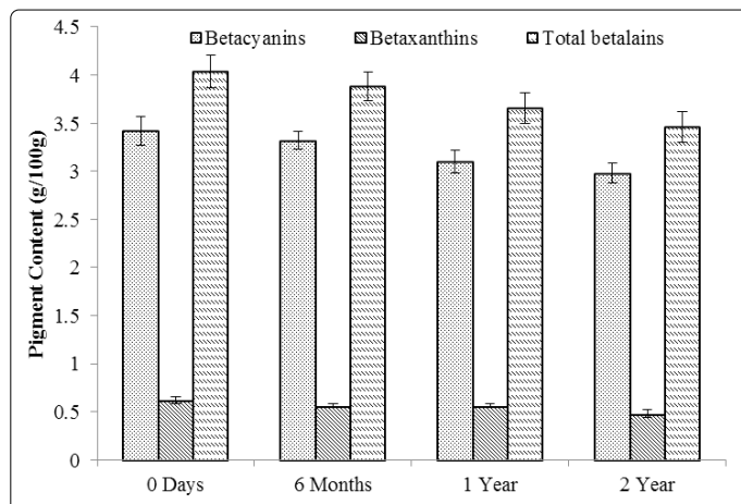
Figure 3. Total betalain content of maltodextrin encapsulated betalain powder from fruits of B. rubra . Vales are mean \pm SD of three replicates.
