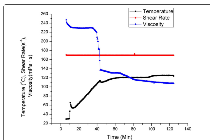
Figure 4. Rheological change of the micro-emulsion fracturing fluid under 120°C and 170s -1 shearing rate.
