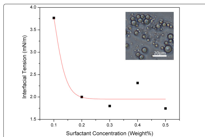
Figure 3. Interfacial tension between the diesel oil and water interface with different concentrations of surfactants. The red line represents the fitted result with lognormal model. Four data points from right side, 0.2%, 0.3%, 0.4%, 0.5%, respectively, showed interfacial tension reached a plateau. Thus we conclude the concentration of surfactant already reached their critical micelle concentration (CMC). Insert is microscopic image of micro-emulsion with 3:7 oil to water ratio and 0.5 w.t. % surfactant.
