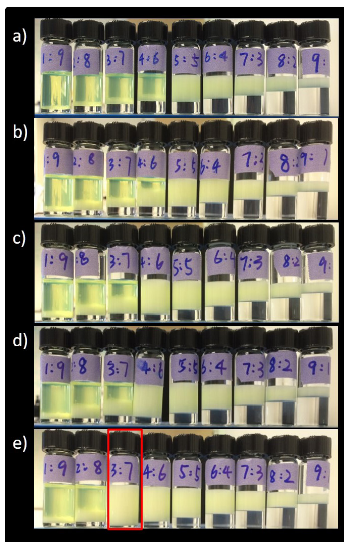
Figure 2. Phase behaviour scanning. From left to right, the oil to water ratio descends as labeled on the vials. Surfactant concentrations were 0.1%, 0.2%, 0.3%, 0.4%, 0.5% for row a), b), c), d), e), respectively. Pictures were taken after samples had been set still for 1 week. A Winsor IV type emulsion (marked as red in picture) was chosen to make the fracturing fluids.
