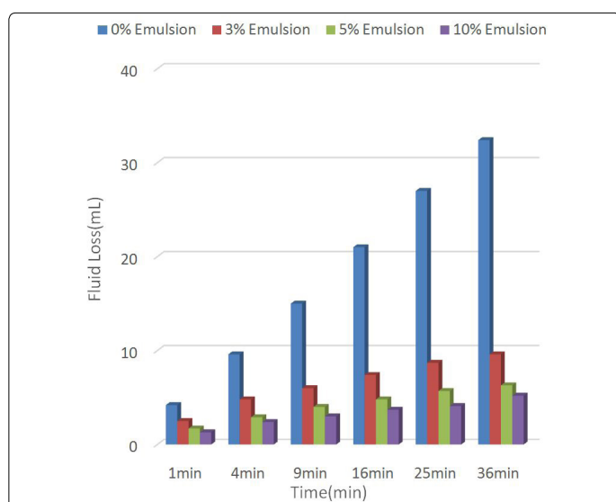
Figure 5. Fluid loss for different fracturing fluid fomulas with different micro-emulsion percentages.
