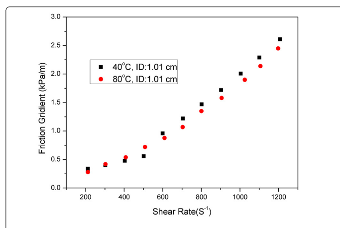
Figure 6. Tube friction profiles with 0.46cm, 1.01cm tubings, under 40°C and 80°C.
