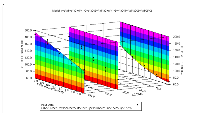
Figure 12. Indicate the results model for both source Iraqi and Foreign RLDPE for Modulus property due to base Tensile Strength property.
