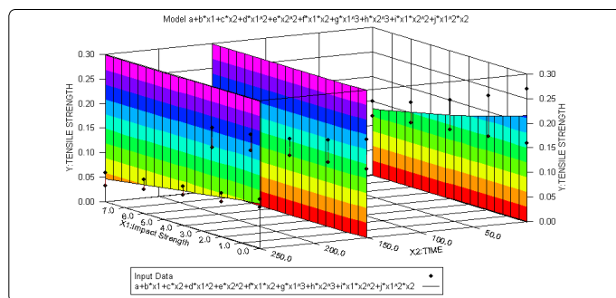
Figure 7. Indicate the model fitted data for impact strength property for both Iraqi and Foreign (RHDPE) due to best fit property tensile strength.
