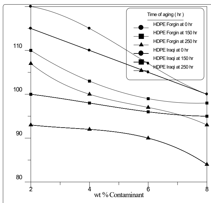
Figure 13. Indicate the Experimental Data for RHDPE
