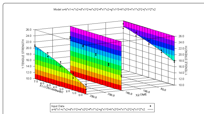
Figure 3. Indicate the theoretical fit model data for RHDPE
