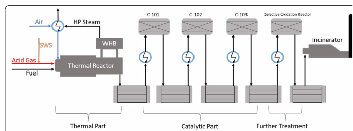
Figure 1. Modified Claus Process for acid gas with ammonia treatment.
