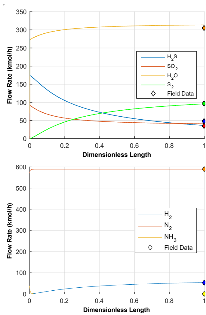
Figure 2a. H 2 S, SO 2 , H 2 O and S 2 ; (b) H 2 , N 2 and NH 3 composition profiles along the Reaction Furnace (RF)
