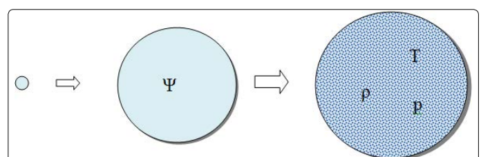
Figure 1. The Transition of the universe from the pure state to mixed.
